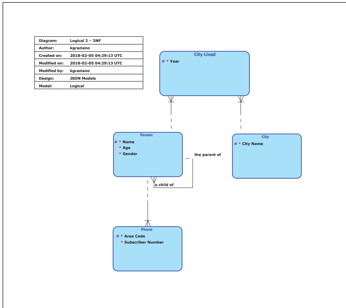
Figure 1—A typical 3NF (third normal form) logical data model
