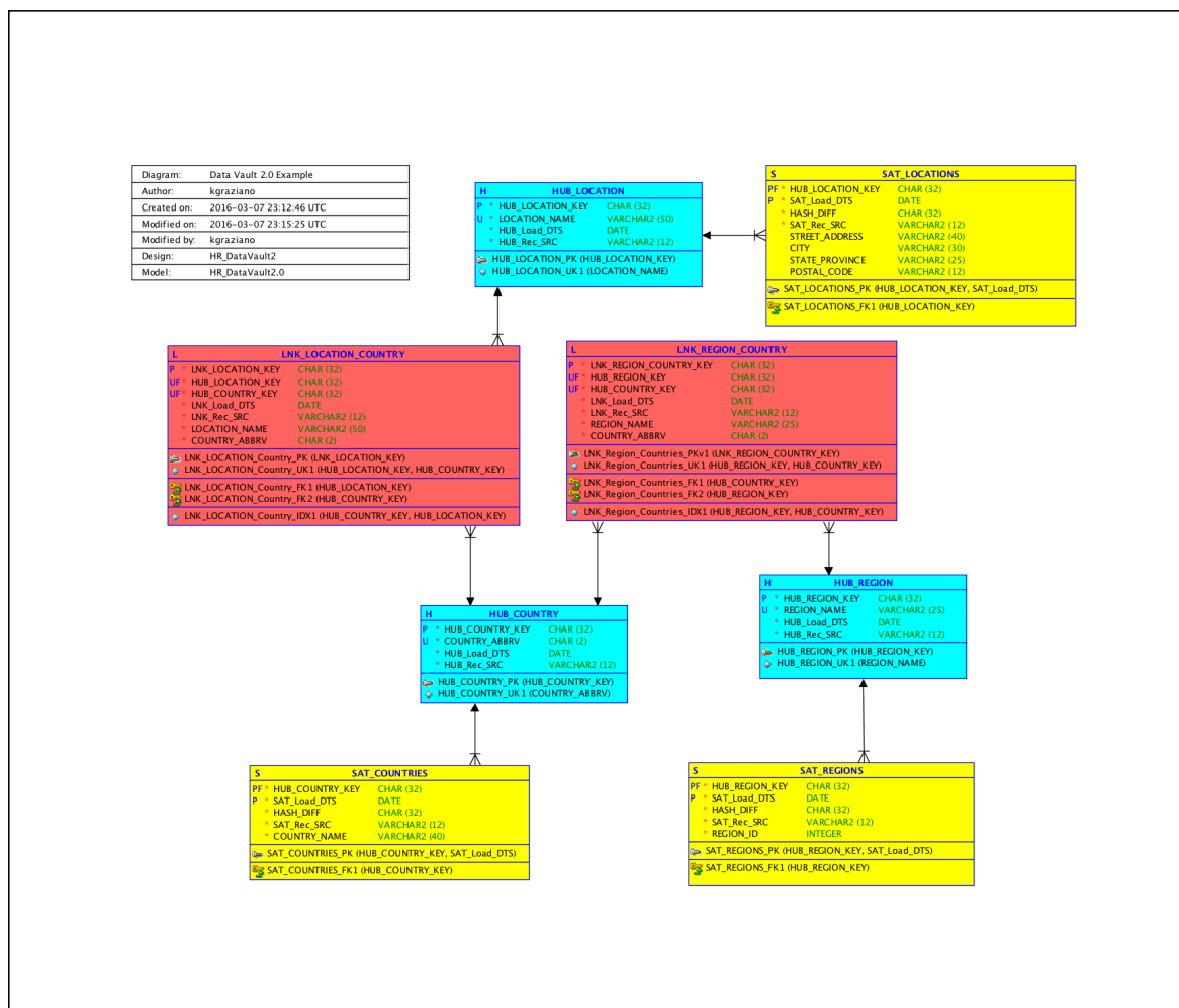
Figure 2—An example data warehouse data model using the Data Vault modeling approach
