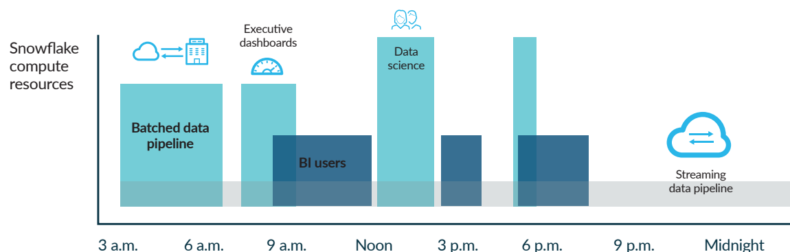
Figure 3: A cloud data platform can support a variety of different workloads and you can allocate them to separate warehouses. The system can process these workloads concurrently without draining resources or degrading performance, so decision-critical information is delivered without delay.
